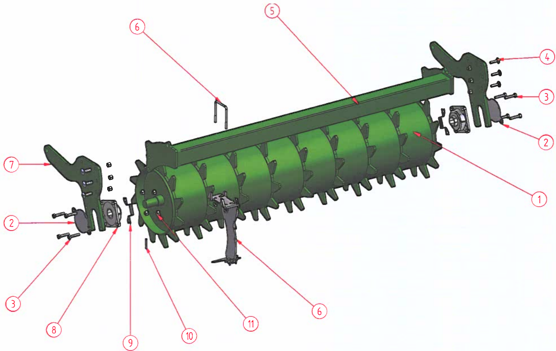
RULLO PACKER Ø324 - PACKER ROLLER Ø324
