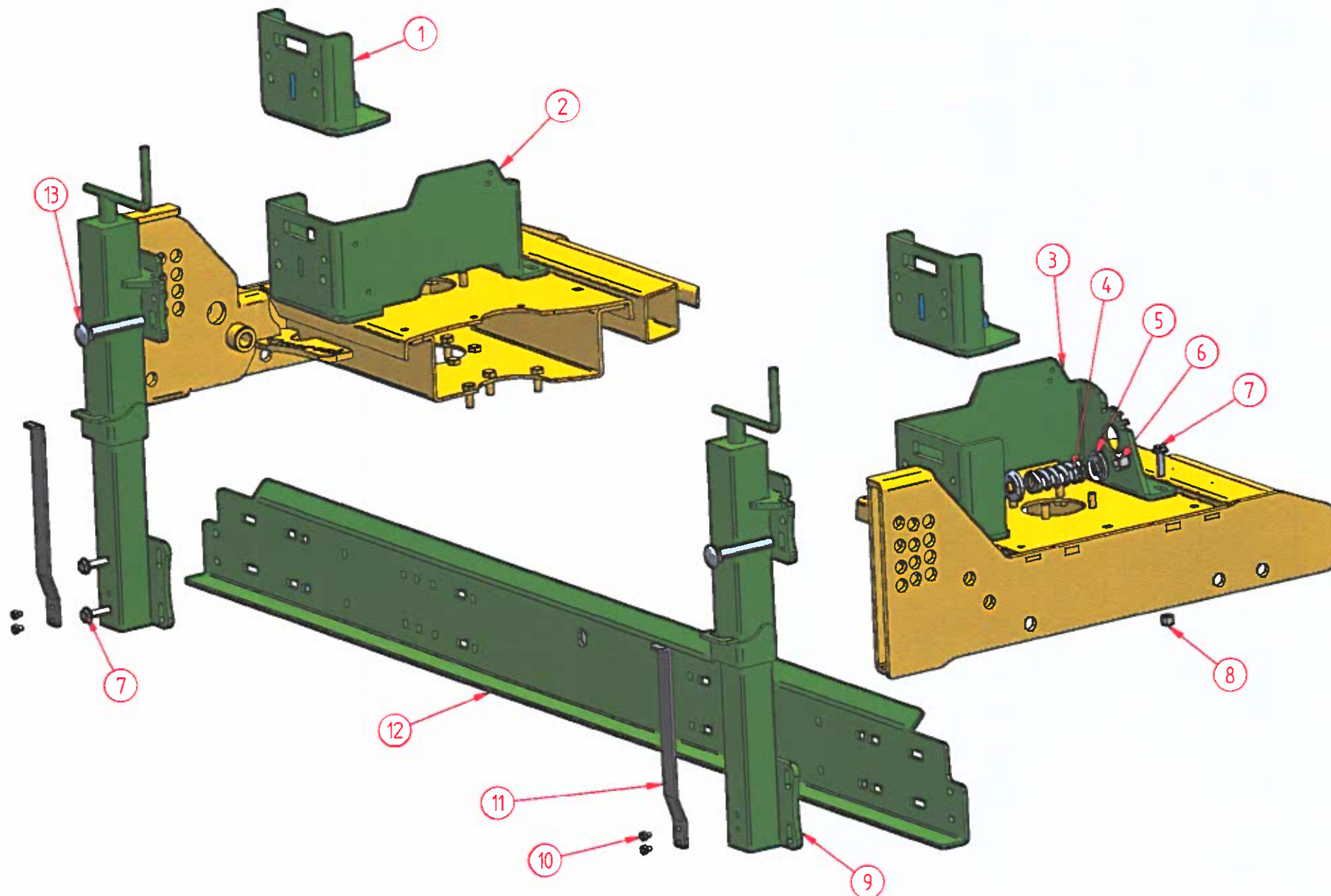
BARRA POSTER. ERPICI FISSI - BAR HANDLE'S CONNECTION
