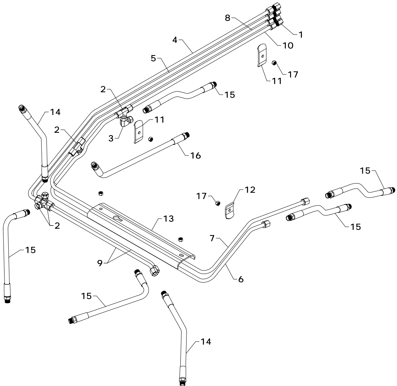
TA-26 & TA-26 PLUS HYDRAULIC LINES
