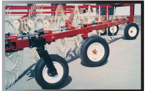
An optional set of 15" front gauge wheels for the 14 Wheel Hi-Capacity rakes help improve float over irrigation tracks or rough ground.
