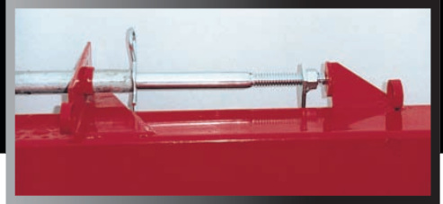
The adjustment for the ground pressure on the rake wheels allows the operator to fine tune the 12, 14 wheel Hi-Capacity rakes to fit varying conditions.
