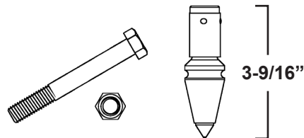
Bullet Tooth & Pilot Hardware Tooth PN 200281 $28.00 Pilot Nut PN 7733 $0.32 Pilot Bolt PN 10123 $1.41
