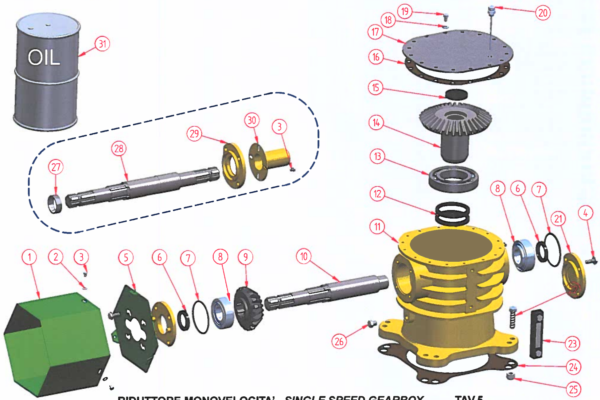
RIDUTTORE MONOVELOCITA' - SINGLE SPEED GEARBOX TAV.5
