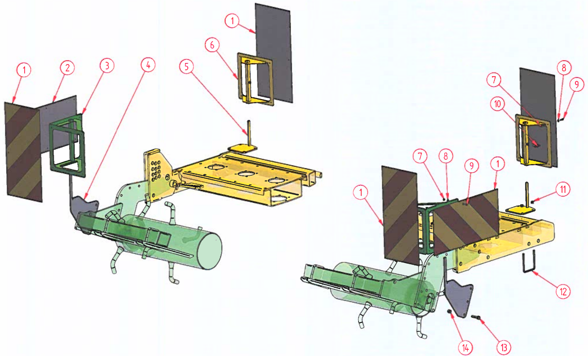
KIT PANNELLI STRADALI - SPACE REPORTING PANEL SUPPORT
