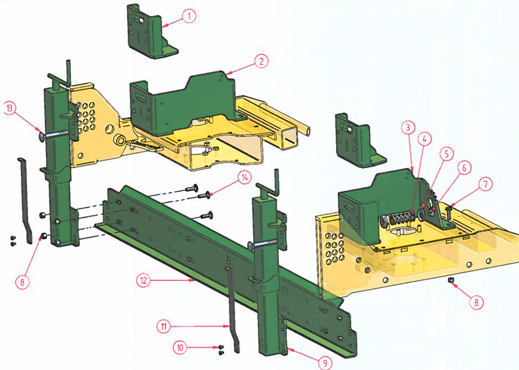
BARRA POSTER. ERPICI FISSI - BAR HANDLE'S CONNECTION
