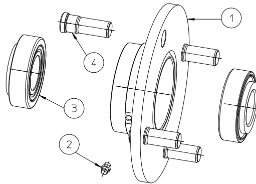
IDLER HUB 270.275
