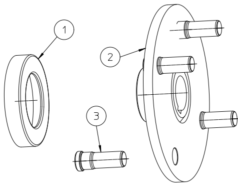
MOTOR HUB 270.274
