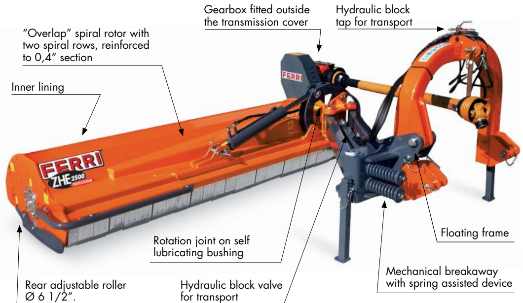
Mechanical breakaway with spring assisted device.
